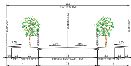
STREET TYPE A - TYPICAL CROSS SECTION
