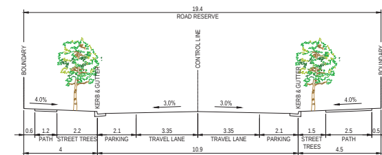
STREET TYPE C - TYPICAL CROSS SECTION
