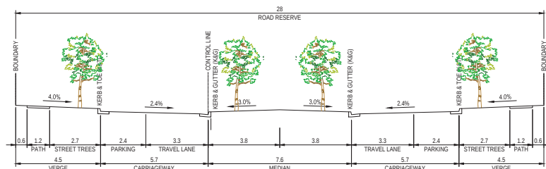
STREET TYPE E - PROMONTORY DRIVE - TYPICAL CROSS SECTION
