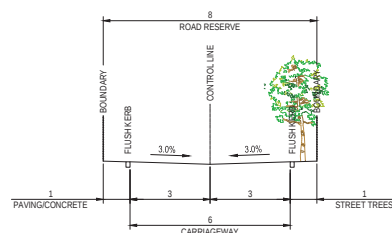
STREET TYPE B - TYPICAL CROSS SECTION
