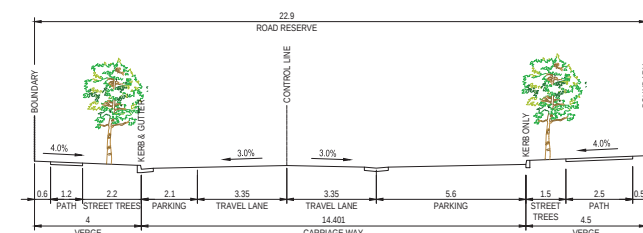
STREET TYPE D - TYPICAL CROSS SECTION
